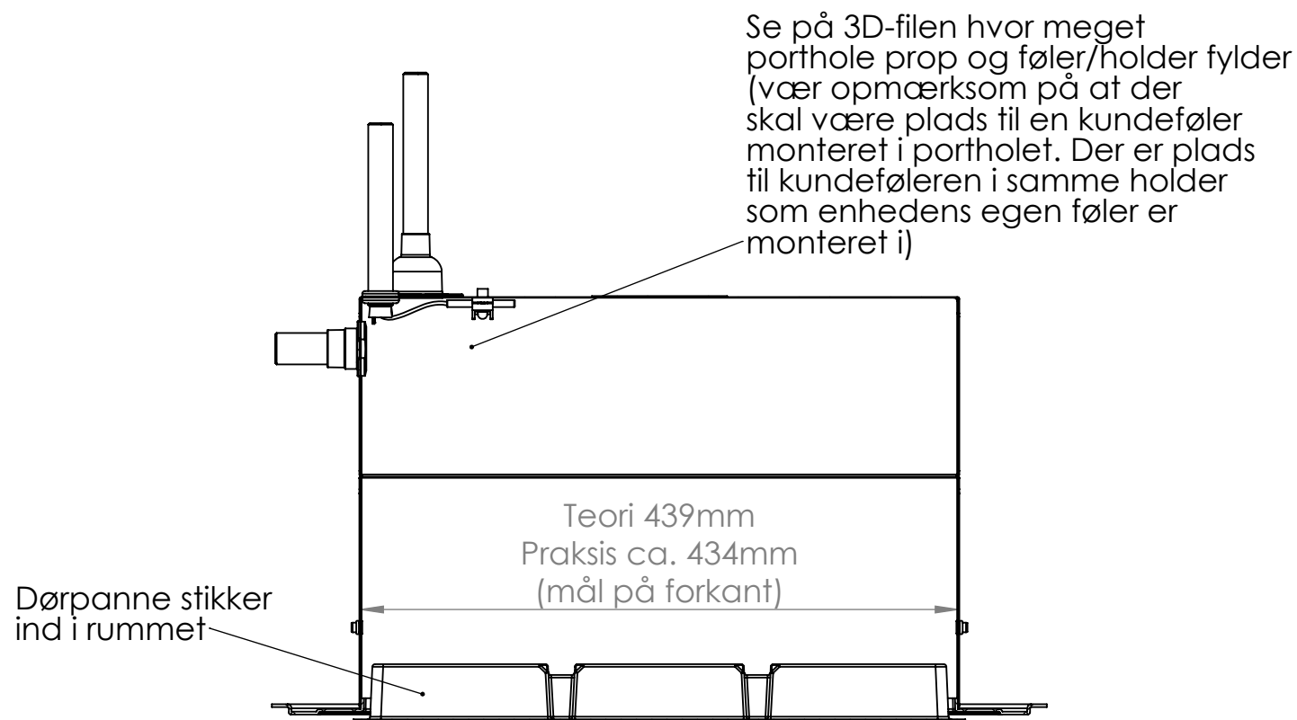
SECTION B-B
