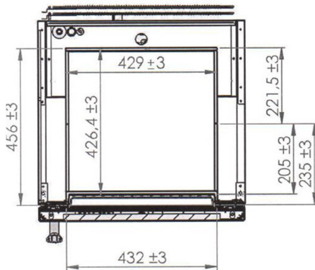
SECTION B-B
